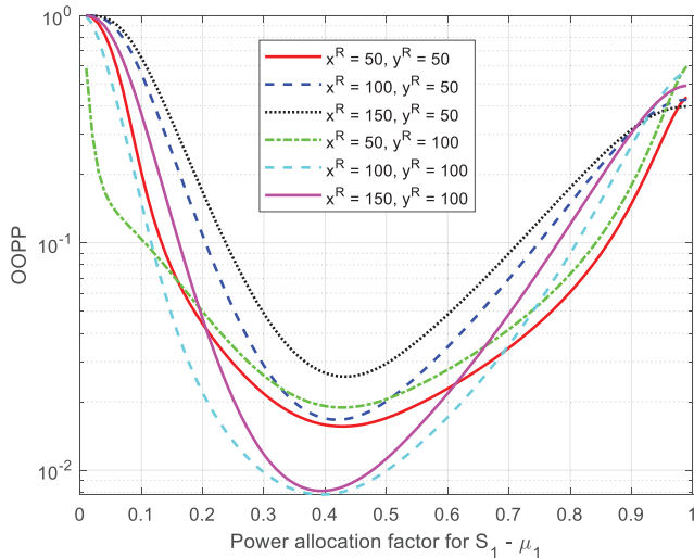
Fig. 5. The OOPP versus UAV position and power allocation for the FNRP ( \mathcal{R} is closer to \mathcal{D} with bigger x^{\mathcal{R}} , \mathcal{R} is further away from jammers with bigger y^{\mathcal{R}} ).
