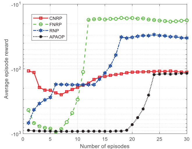
Fig. 7. Training progress for the four protocols.
