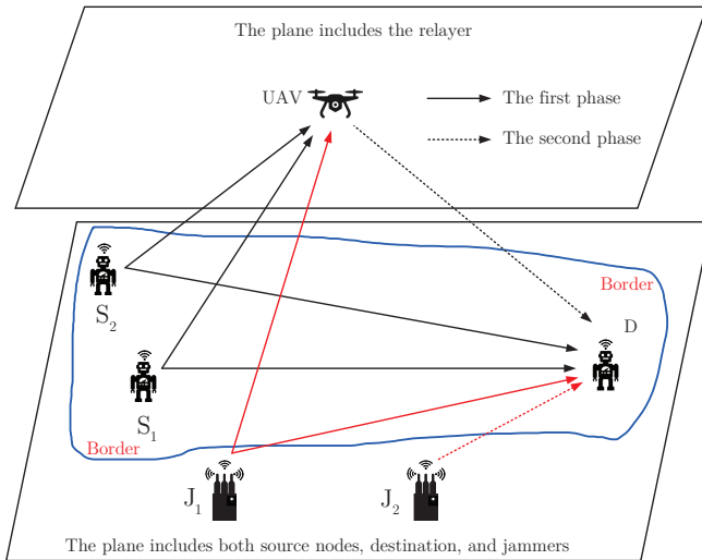
Fig. 1. System model.
