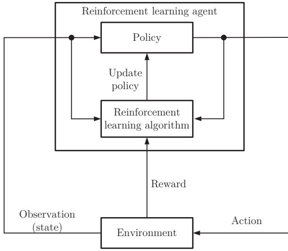
Fig. 2. Reinforcement learning architecture.
