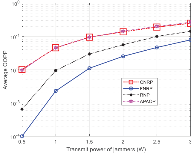
Fig. 8. Effect of transmit power levels of both jammers on average OOPP in the inference phase when P_{\mathcal{J}_1} = P_{\mathcal{J}_2} .
