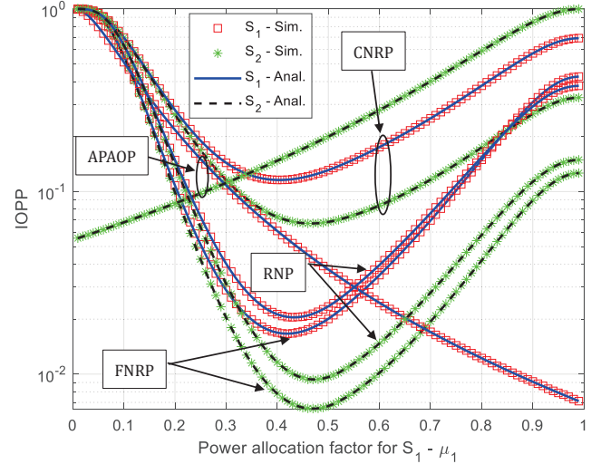
Fig. 3. The IOPP for each source node taking both phases into account.
