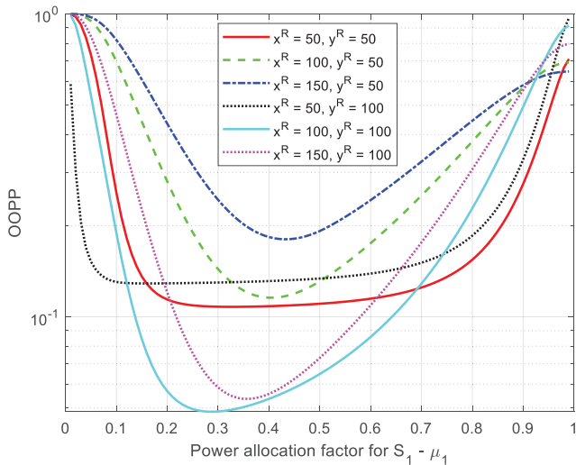
Fig. 4. The OOPP versus UAV position and power allocation for the CNRP ( \mathcal{R} is closer to \mathcal{D} with bigger x^{\mathcal{R}} , \mathcal{R} is further away from jammers with bigger y^{\mathcal{R}} ).
