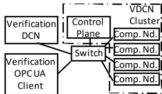
Fig. 4. Testbed deployment.
