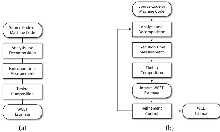
Figure 1: Traditional MBTA work-flow (a) versus the FORTAS work-flow (b).
