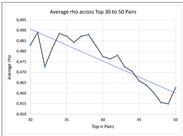
Fig. 8: Average correlation coefficient across top-30 to top-50 pairs
