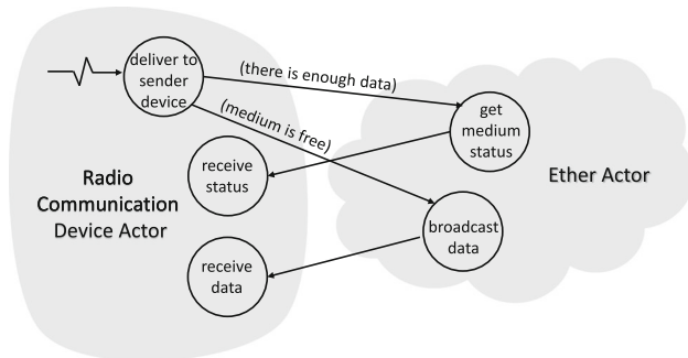
Fig. 4 How events of wireless communication mechanism are associated with actors
