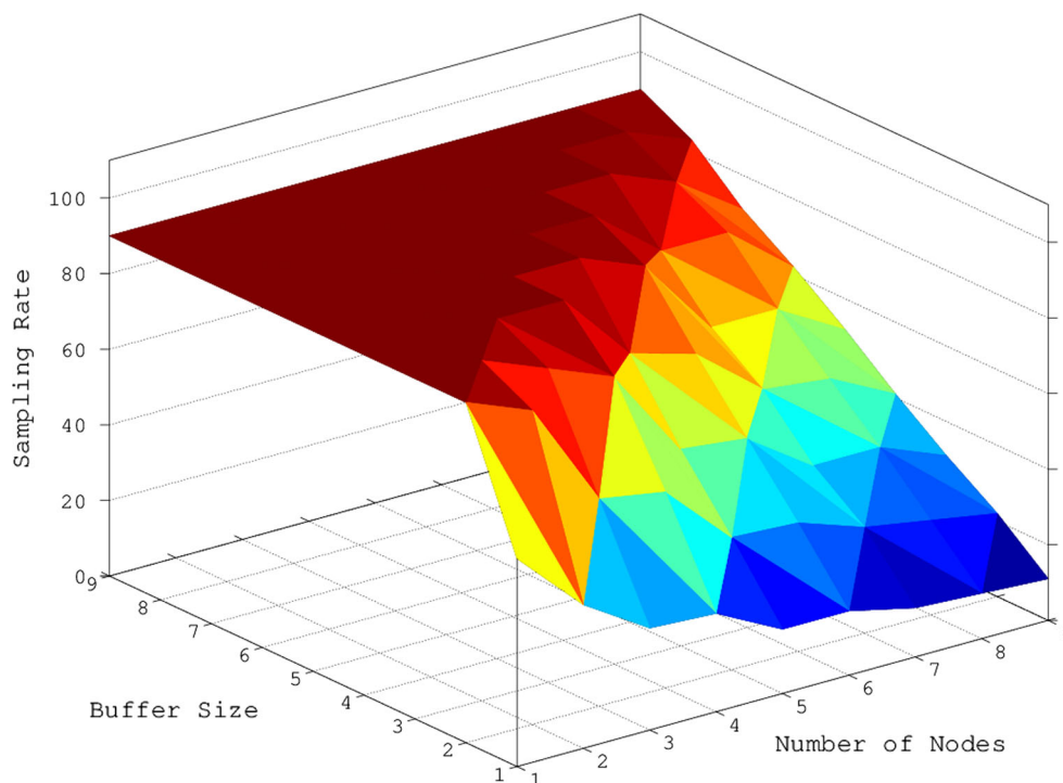
Fig. 6 The maximum sampling rate in case of using TDMA protocol and setting the value of sensorTaskDelay to 2ms
