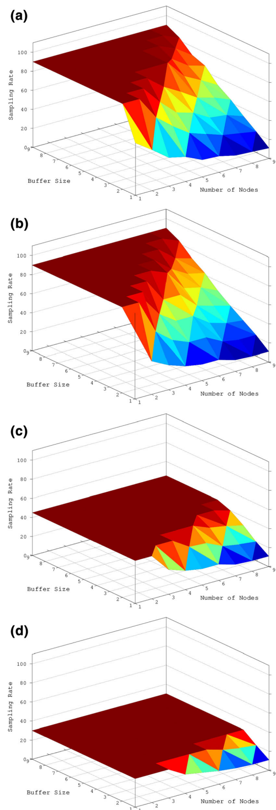
Fig. 7 Maximum possible sampling rate in case of different communication protocols, number of nodes, sensor internal task delays, and radio packet size. a TDMA, sensor task delay is 5 ms. b TDMA, sensor task delay is 10 ms. c TDMA, sensor task delay is 20 ms. d TDMA, sensor task delay is 30 ms
