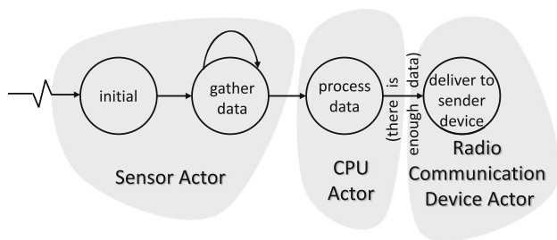
Fig. 3 How events of a WSAN sensor are associated with actors
