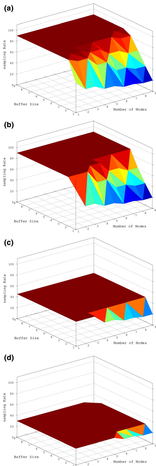
Fig. 8 Maximum possible sampling rate in case of different communication protocols, number of nodes, sensor internal task delays, and radio packet size. a B-MAC, sensor task delay is 5 ms. b B-MAC, sensor task delay is 10 ms. c B-MAC, sensor task delay is 20 ms. d B-MAC, sensor task delay is 30 ms
