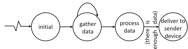
Fig. 2 The event graph of a WSA sensor behavior
