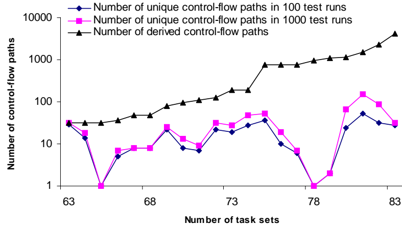
Figure 5.6: This graph shows the number of found system level control-flow paths in 1000 test runs and 100 test runs compared to the number of derived paths in task sets that are considered to have significant execution time slack.
