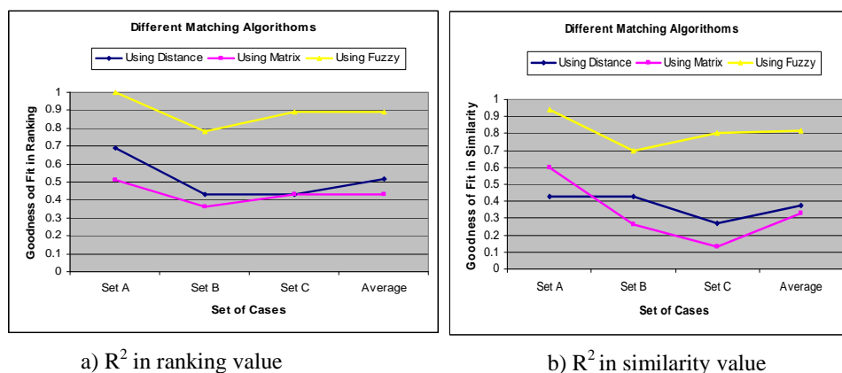
Fig. 6. Comparison among three different matching algorithms.
