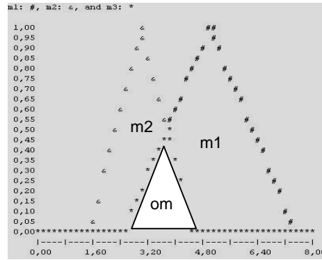
Fig. 5. Fuzzy similarity using triangular membership functions
