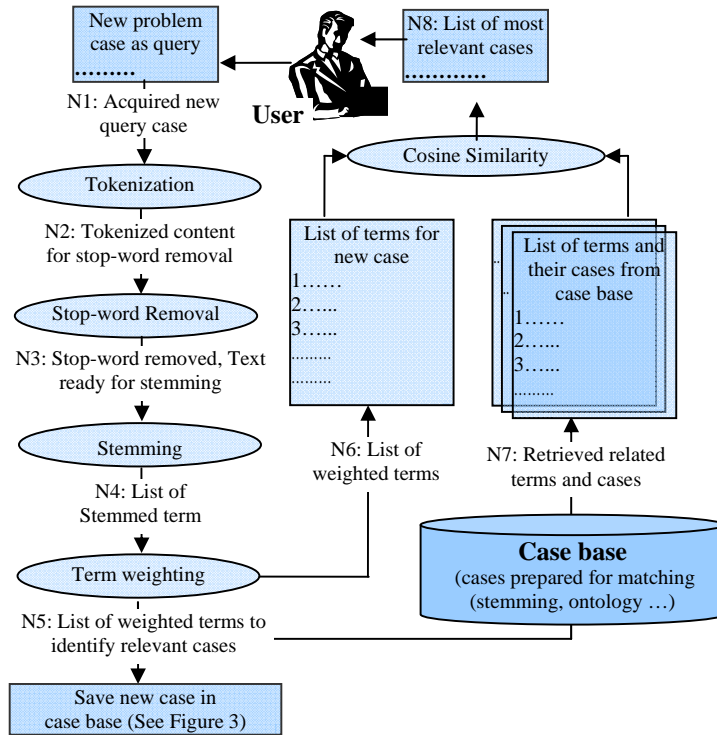
Fig. 2. Work flow diagram of the retrieval process for textual cases
